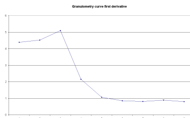
Figure 1. An instance of the derivative of the granulometry curve. This curve exhibits a sharp drop between 3 and 4, which corresponds to half the mean radius of the fibres.
