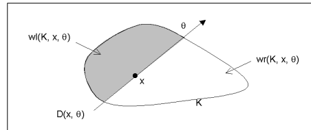
Figure 1. Partition of the convex body K according to the straight line D(x, \theta) .
