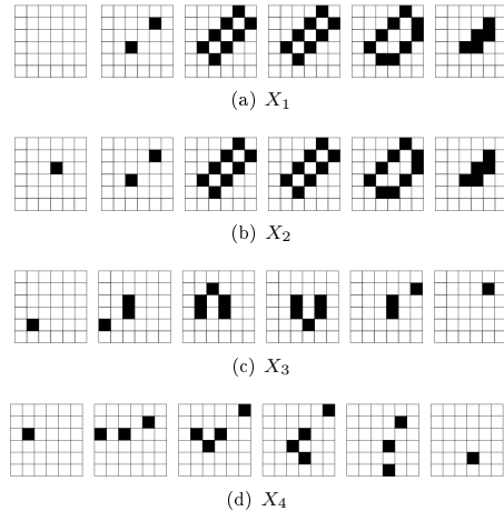
Figure 2. 2D view of X_i ( i = 1 to 4).
